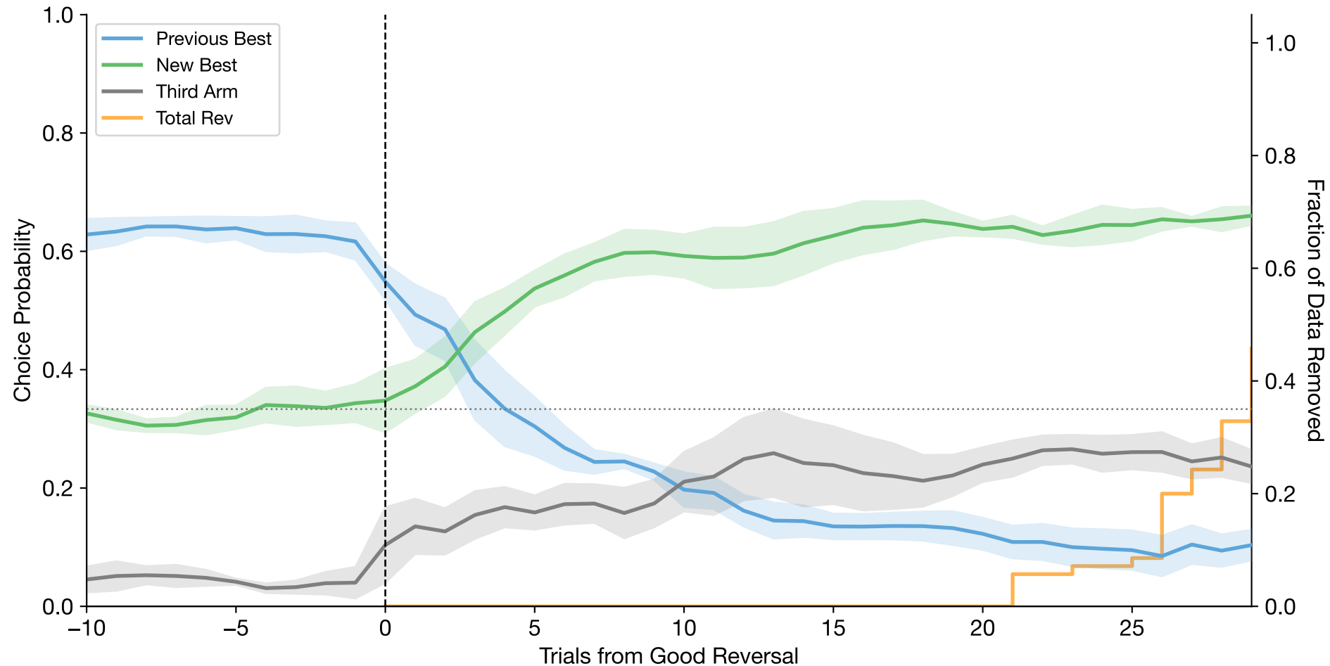
Good Reversal-Aligned Choices (mean \pm se across subjects | n=5 subjects, n=70 reversals)
